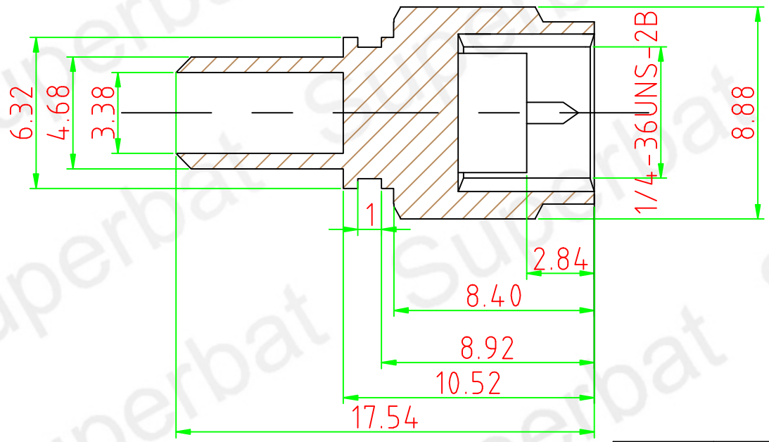
SECTION B-B
