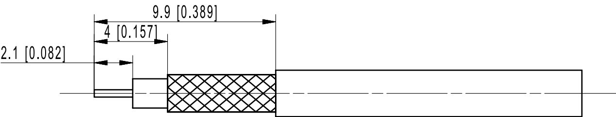
STRIPPING DIMENSIONS
